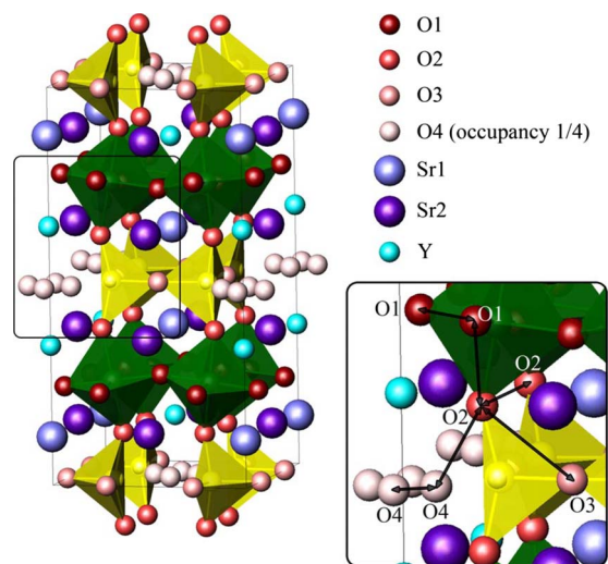
FIG. 1. (Color online) In the crystal structure of \text{Sr}_{0.7}\text{Y}_{0.3}\text{CoO}_{2.62} the \text{CoO}_6 octahedra layers alternate with oxygen-deficient layers that consist of O3, O4 (occupancy factor of \frac{1}{4} ), and Co1 atoms.
